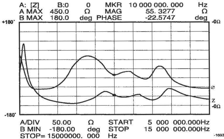
Figure 3-7. rf Output Impedance Versus Frequency
