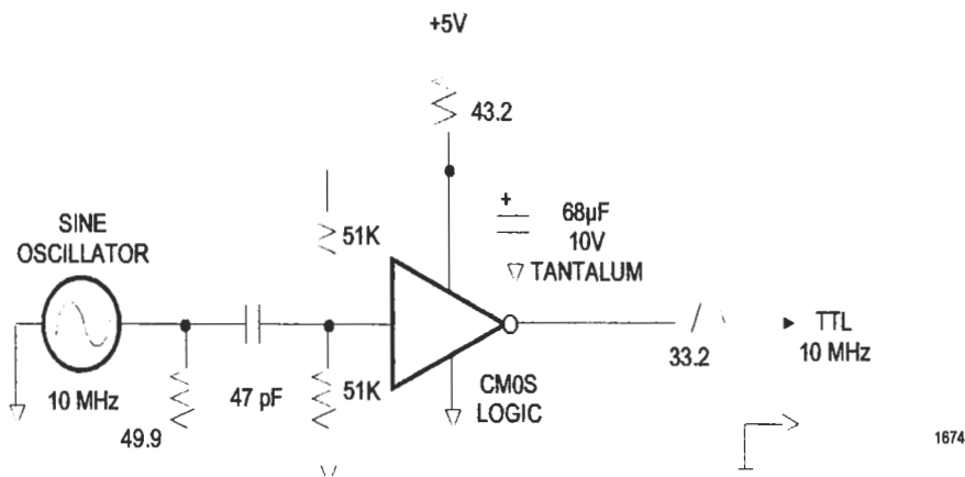
Figure 3-2. Sine-to-TTL Conversion, Using C-MOS Logic, Recommended Approach
