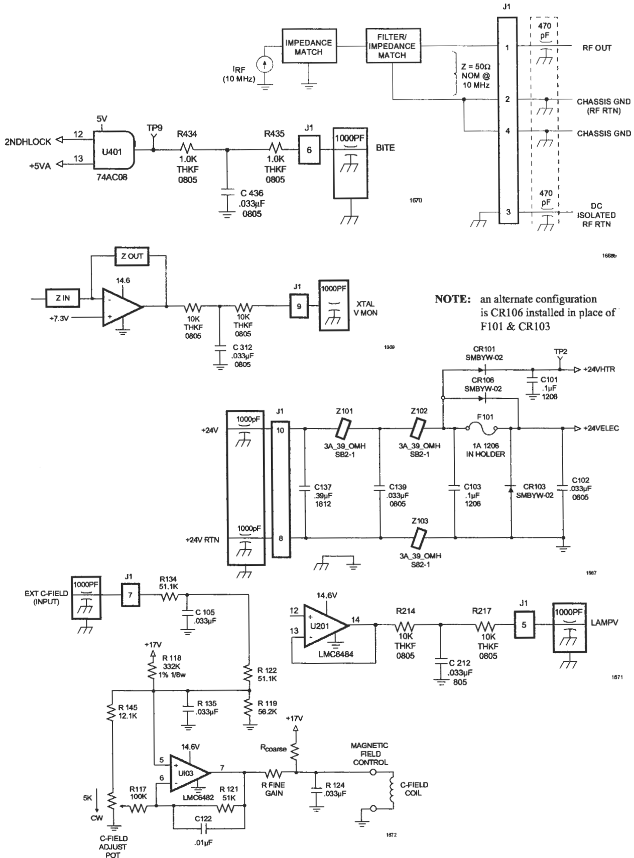
Figure 3-1. Interface Circuitry of LPRO Connector J1
