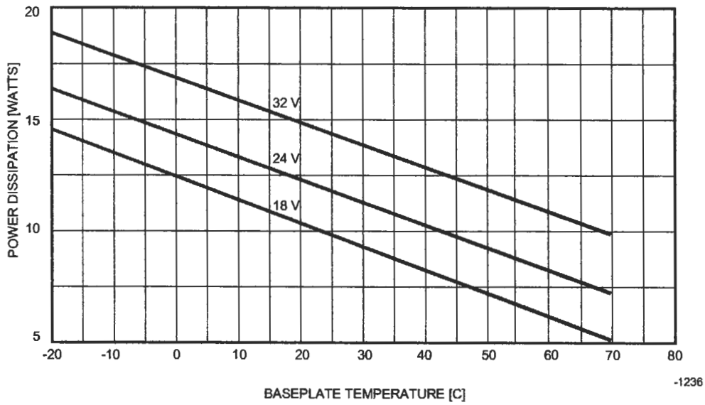
Figure 1-3. Total Unit Power Dissipation, Typical (free convection)
