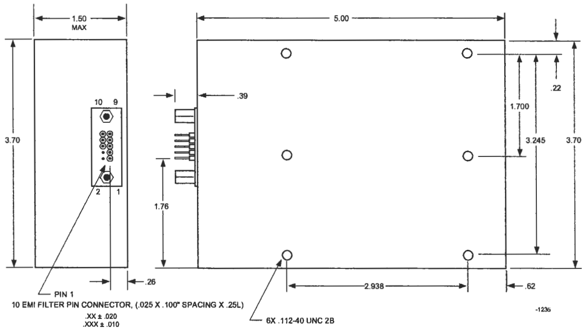
Figure 1-2. Outline Drawing, LPRO
