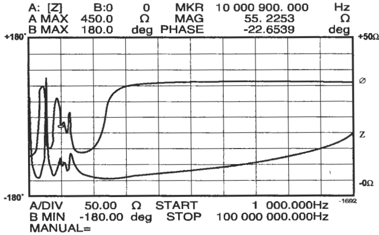
Figure 3-6. rf Output Impedance Versus Frequency
