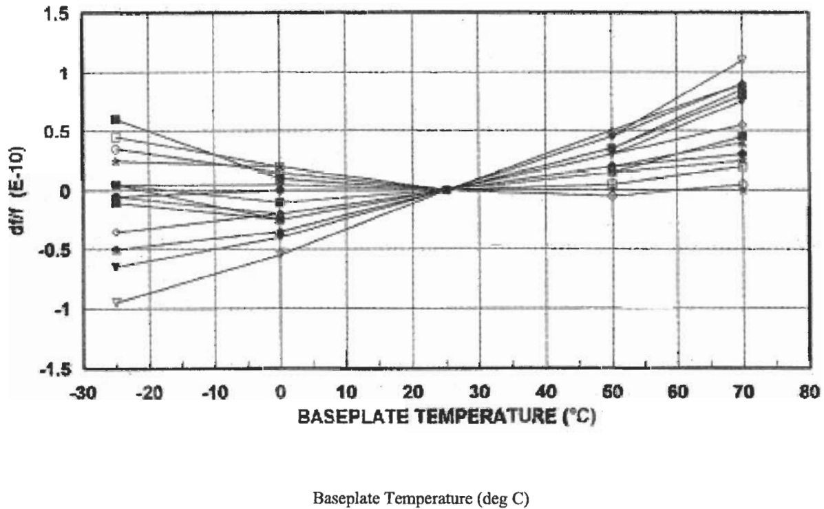
Figure 1-4. Representative LPRO \Delta f/f versus Temperature
