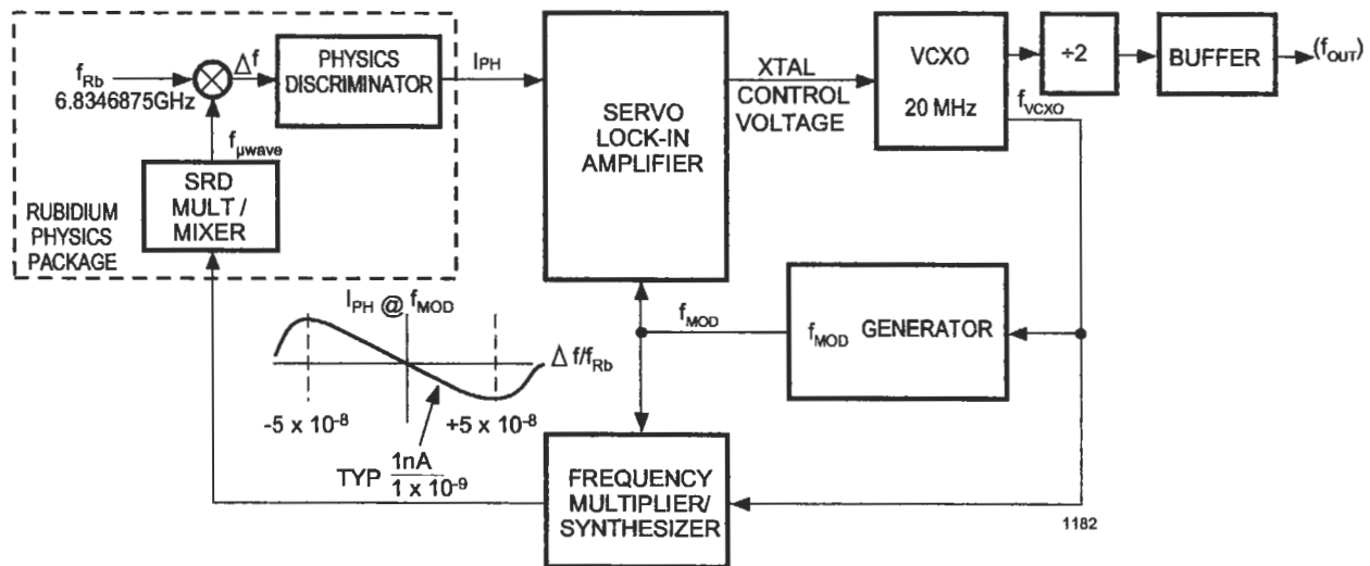
Figure 2-1. LPRO Rb Control Loop Block Diagram
